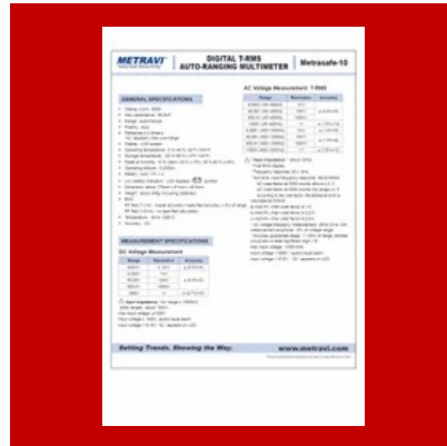
METRAVI METRASAFE -10 DIGITAL MULTIMETER
